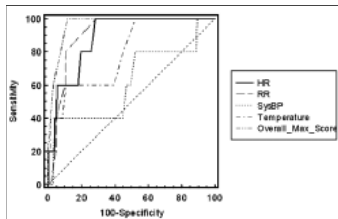
Figure 3. ROC curves for serious outcome (death/ICU admission).
